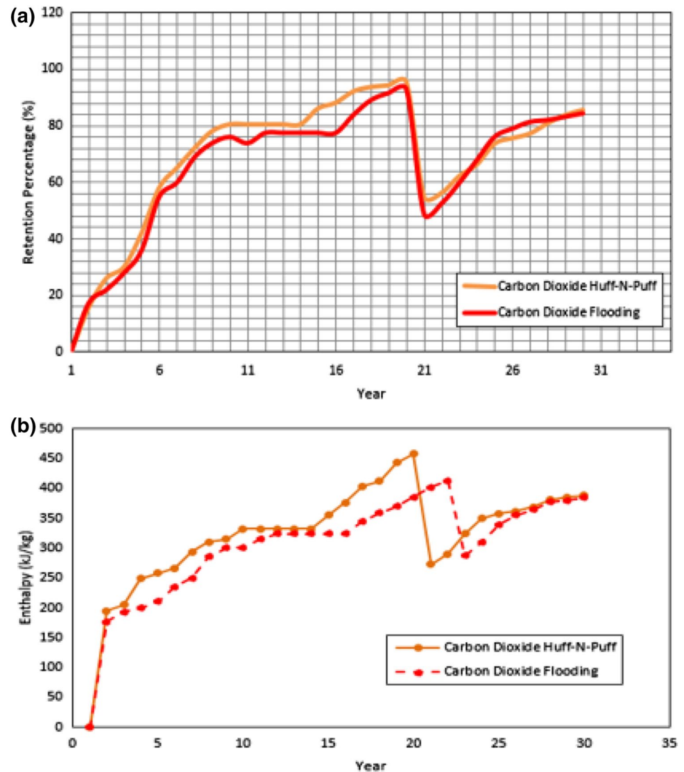
Fig. 11 a CO 2 retention estimation in WCSB Alberta tight gas reservoir, b Subsurface CO 2 retention enthalpy in WCSB Alberta tight gas reservoir
