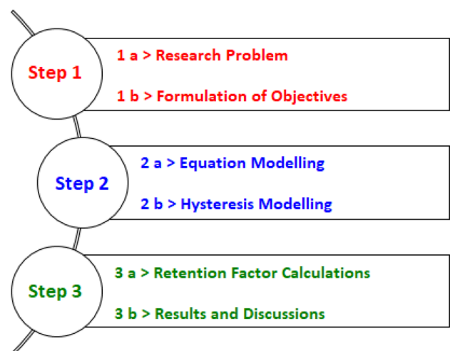
Fig. 8 CO 2 retention mechanism estimation procedure
