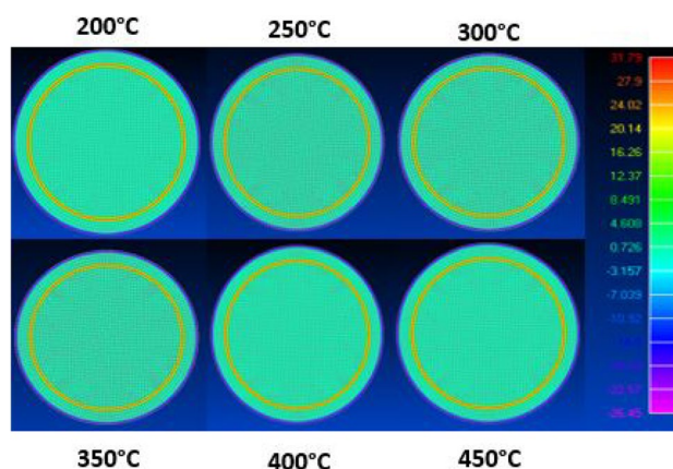
Fig. 8 Thermally constrained load at different steady-state thermal regimes (for the view of figures with labels and coordinates, a reader is advised to see Online Appendix A1)
