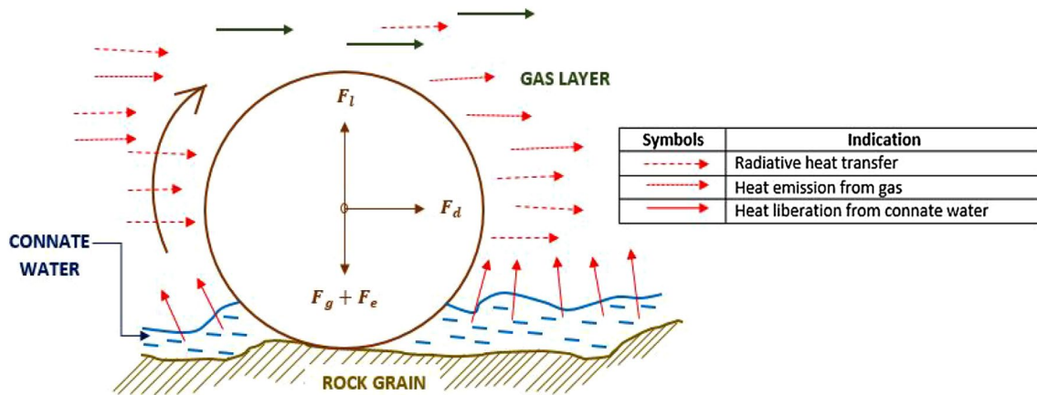
Fig. 2 Attached fine particle under the regime of mechanical forces during gas and heat flow in porous rocks with the presence of connate water. This image is a modified or extended version of Zeinjahromi et al. (2012)
