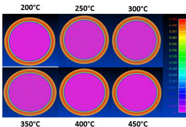
Fig. 6 Heat flux across the well at different steady-state thermal regimes (for the view of figures with labels and coordinates, a reader is advised to see Online Appendix A1)
